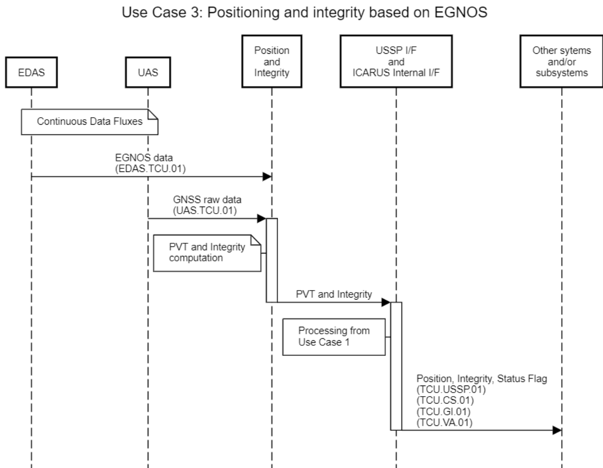
Figure 4-6: Use case 3 sequence diagram
