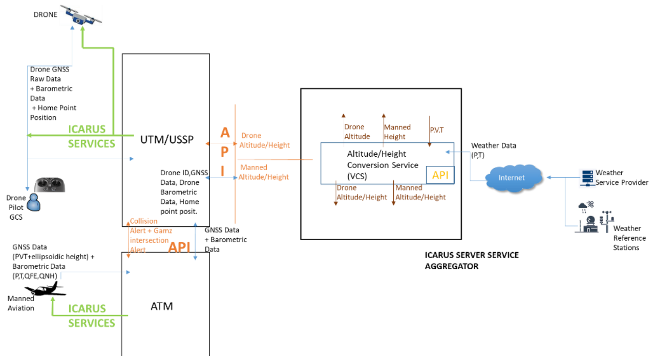
Figure 2-14: VCS high level architecture
