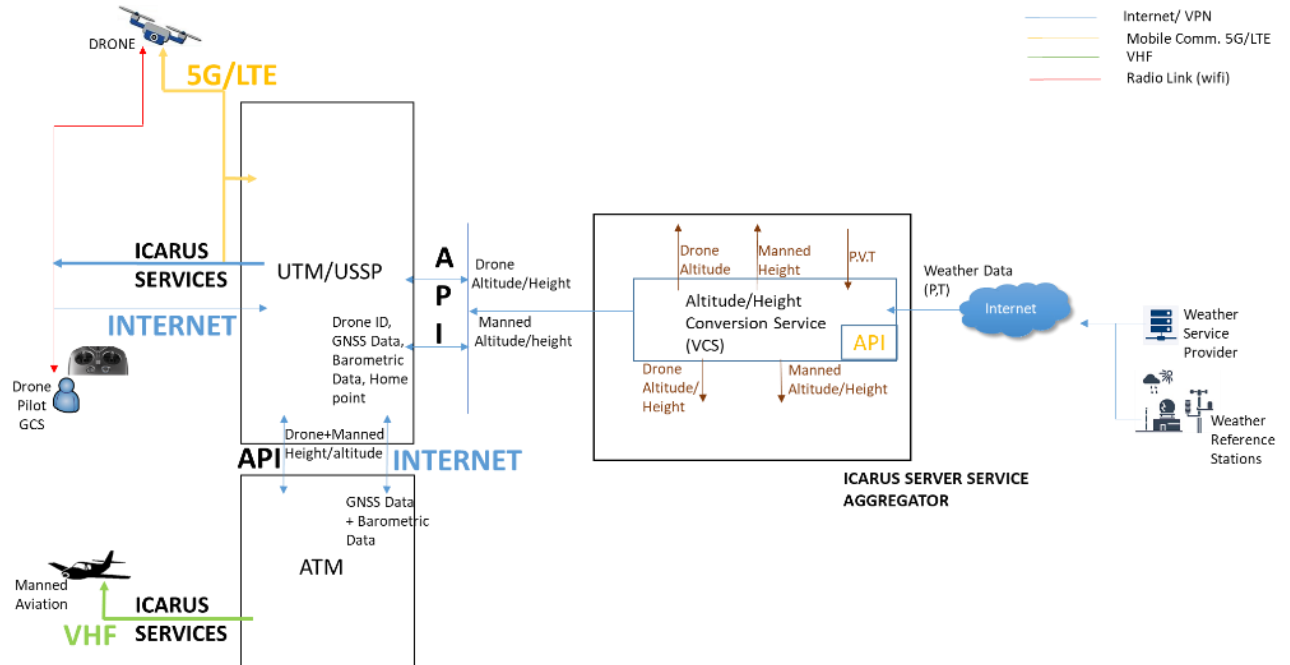
Figure 2-13: Vertical Conversion Service data network infrastructure
