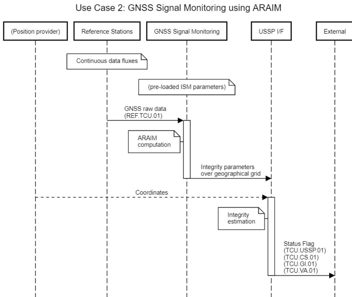
Figure 4-5: Use case 2 sequence diagram
