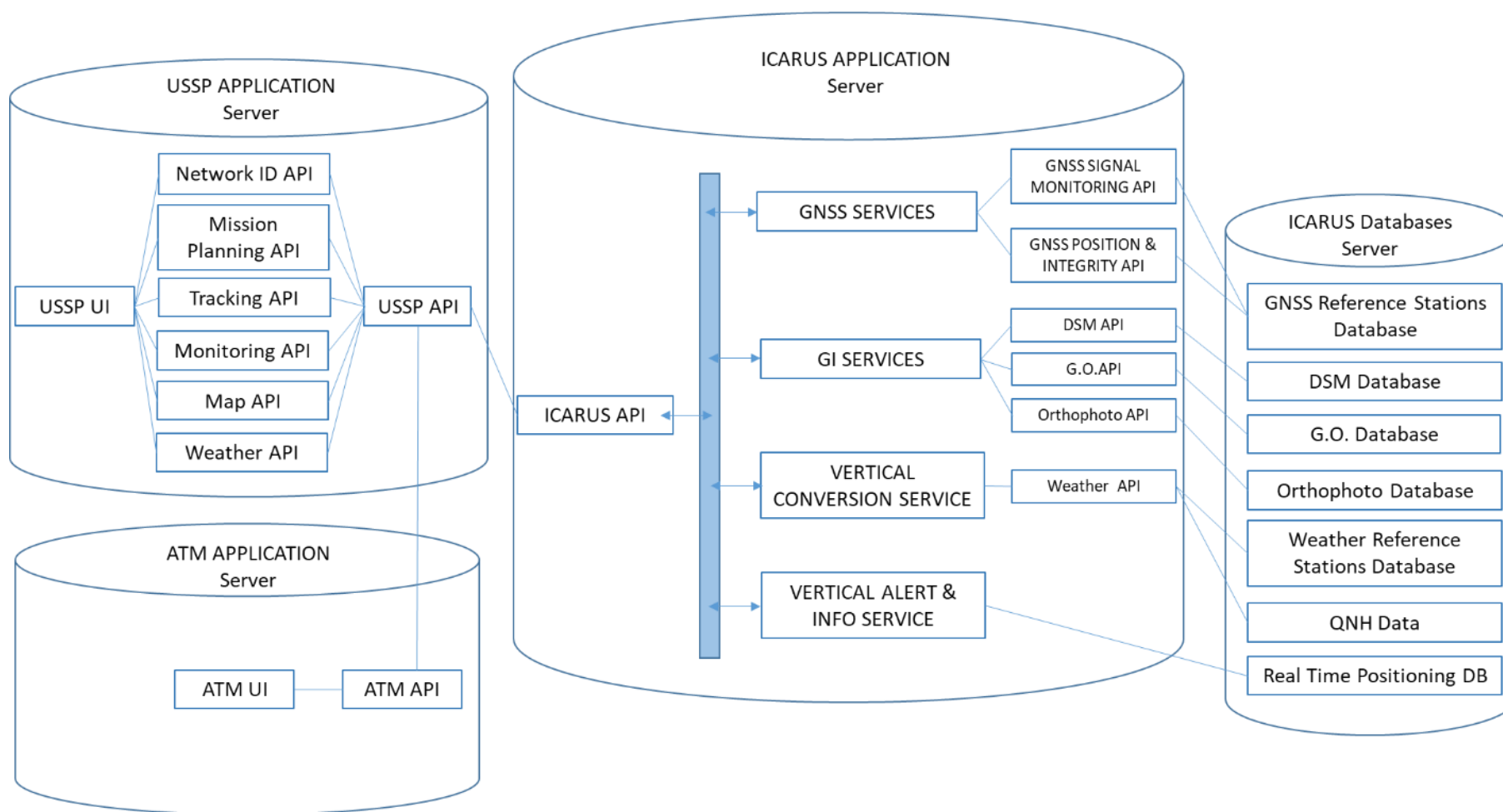
Figure 2-5: ICARUS Components and Micro Services
